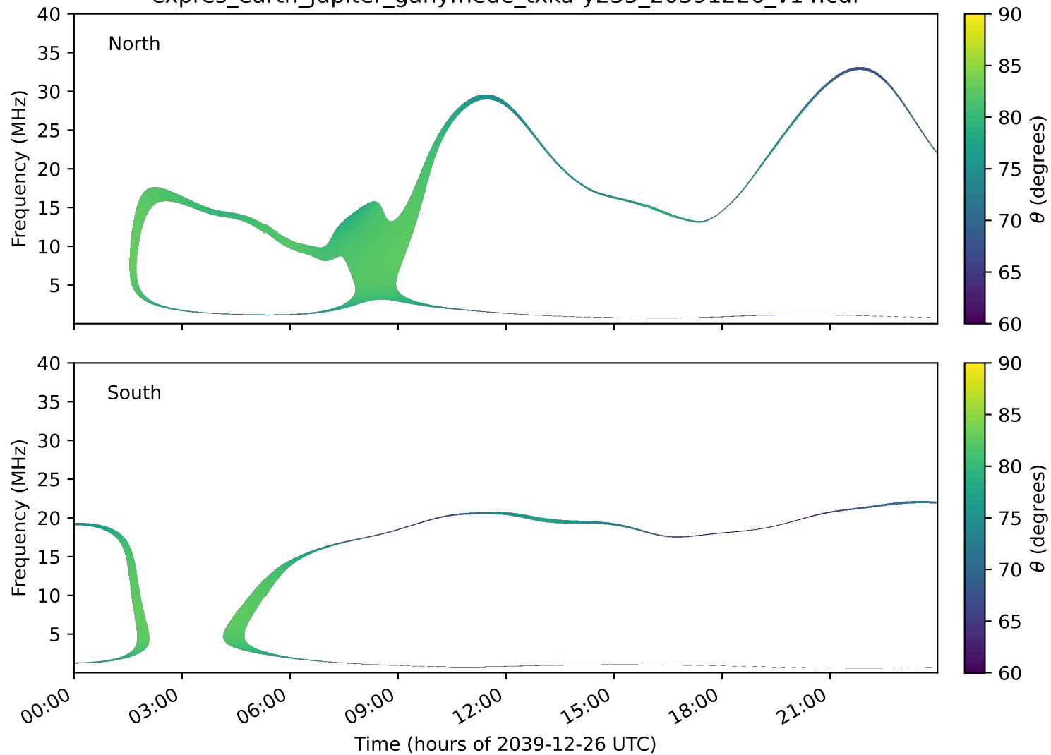
expres_earth_jupiter_ganymede_txka-y235_20391226_v14.cdf
