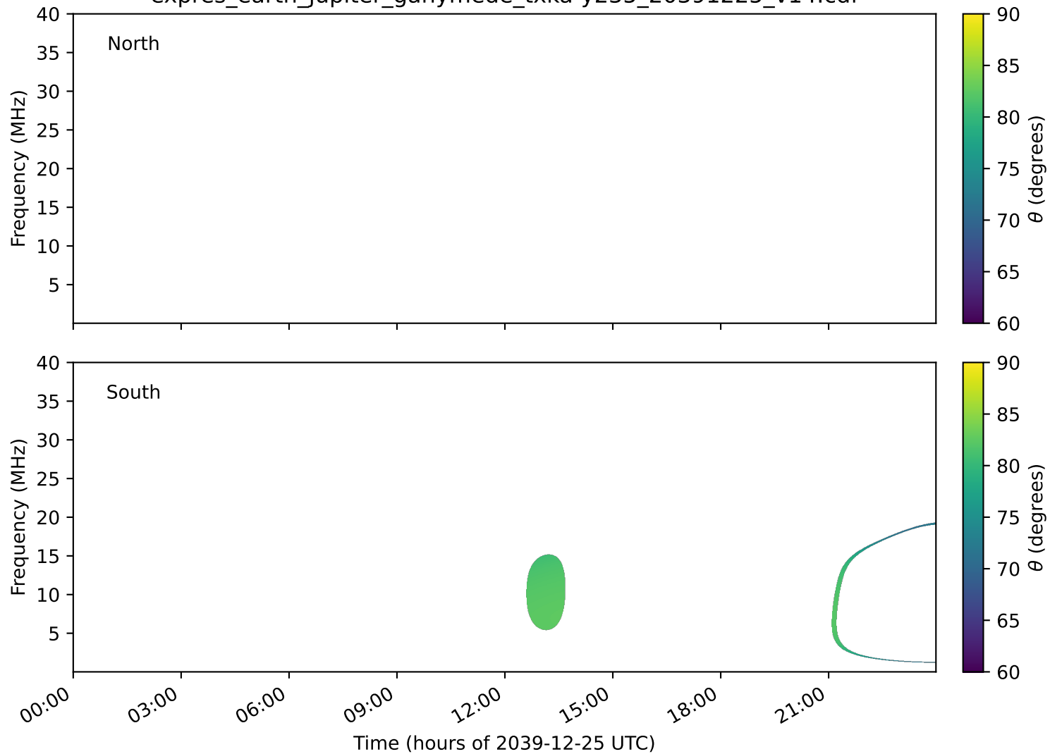
expres_earth_jupiter_ganymede_txka-y235_20391225_v14.cdf
