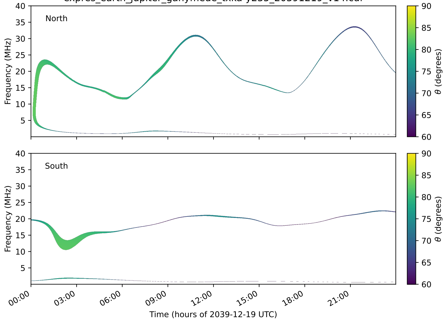
expres_earth_jupiter_ganymede_txka-y235_20391219_v14.cdf
