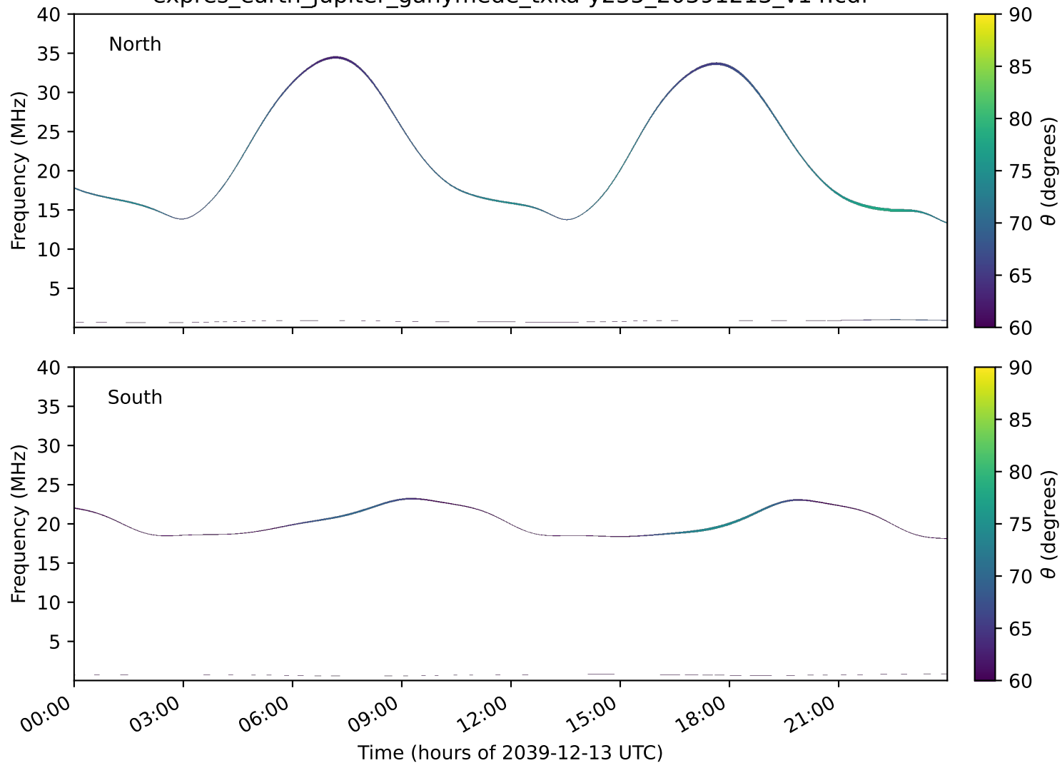
expres_earth_jupiter_ganymede_txka-y235_20391213_v14.cdf
