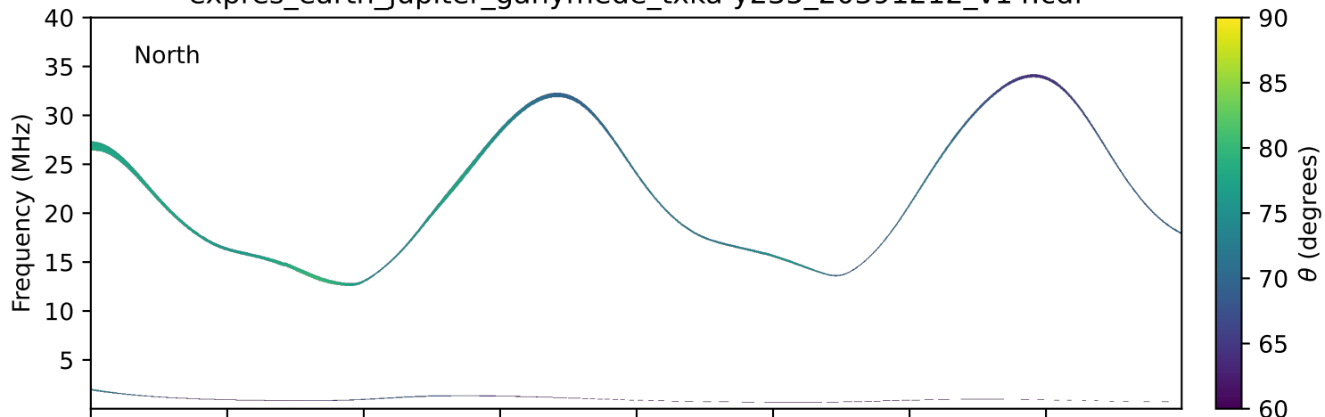
expres_earth_jupiter_ganymede_txka-y235_20391212_v14.cdf
