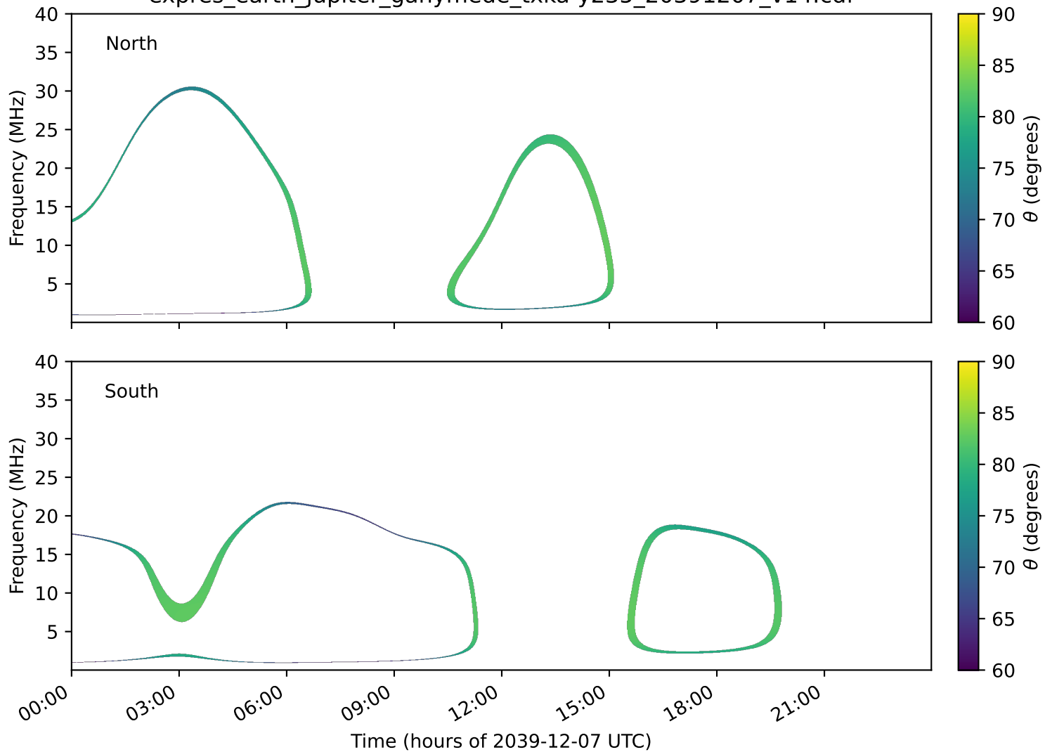
expres_earth_jupiter_ganymede_txka-y235_20391207_v14.cdf
