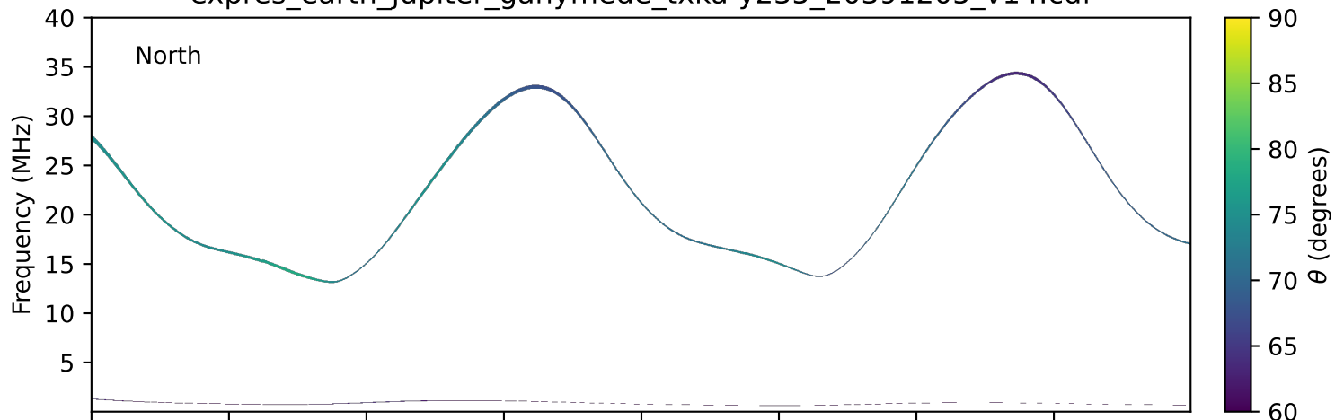
expres_earth_jupiter_ganymede_txka-y235_20391205_v14.cdf
