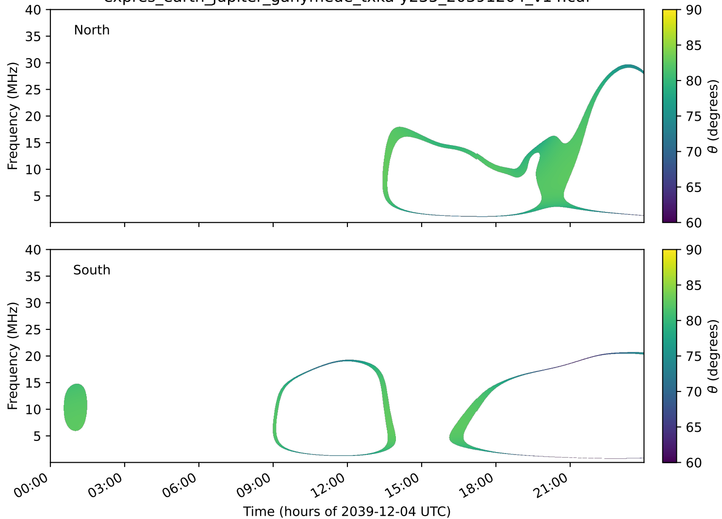
expres_earth_jupiter_ganymede_txka-y235_20391204_v14.cdf
