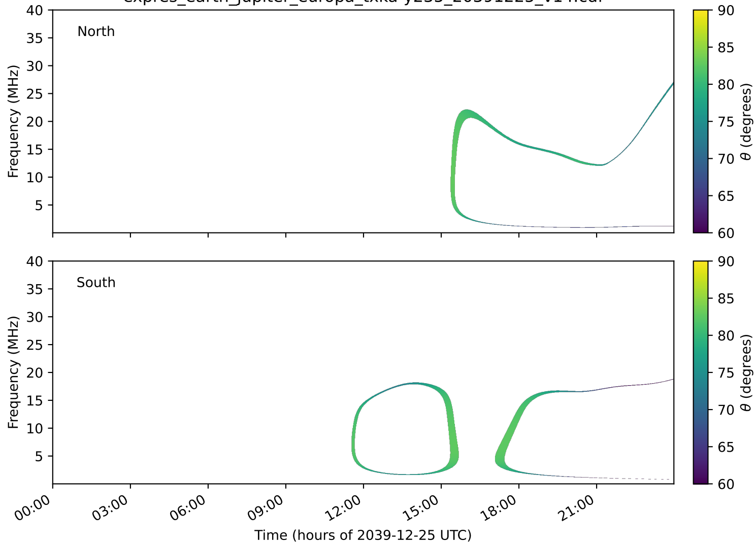
expres_earth_jupiter_europa_txka-y235_20391225_v14.cdf
