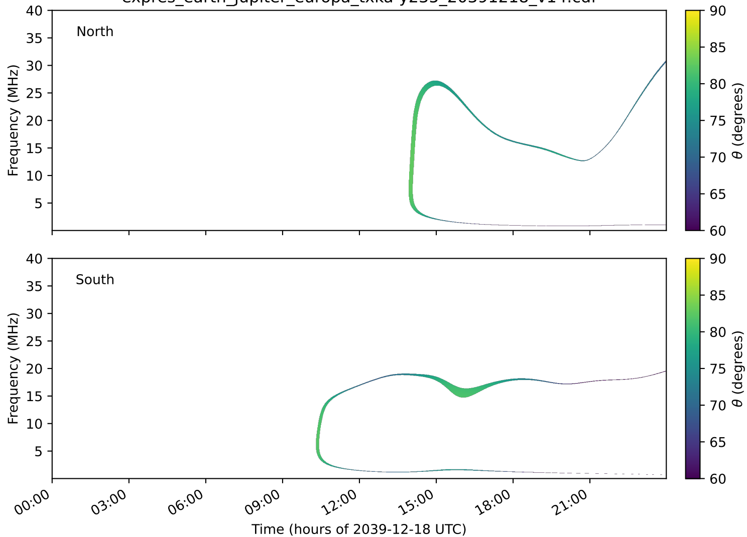
expres_earth_jupiter_europa_txka-y235_20391218_v14.cdf
