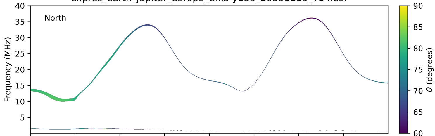
expres_earth_jupiter_europa_txka-y235_20391215_v14.cdf
