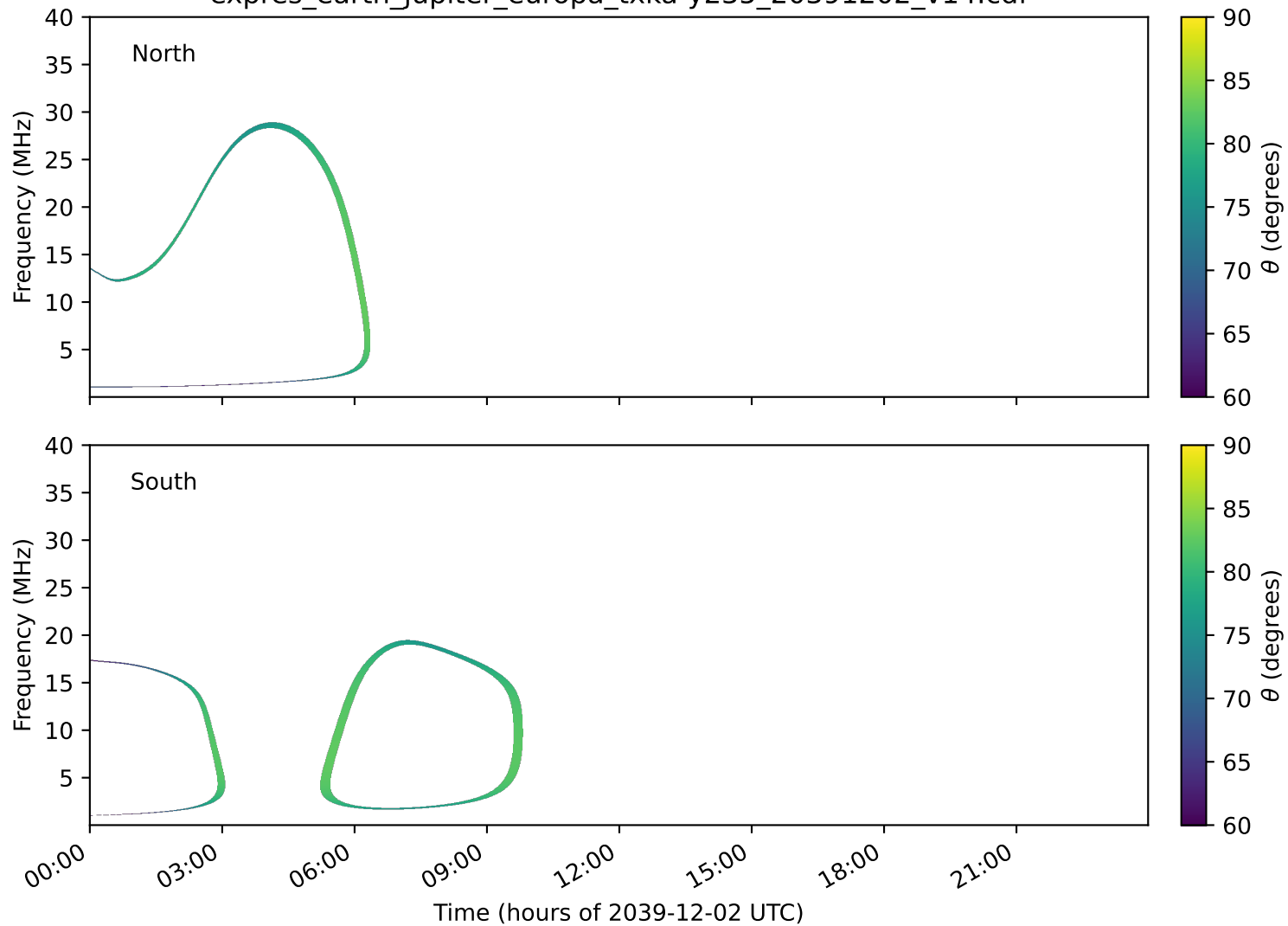
expres_earth_jupiter_europa_txka-y235_20391202_v14.cdf
