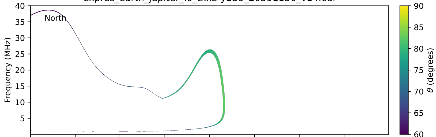
expres_earth_jupiter_io_txka-y235_20391130_v14.cdf
