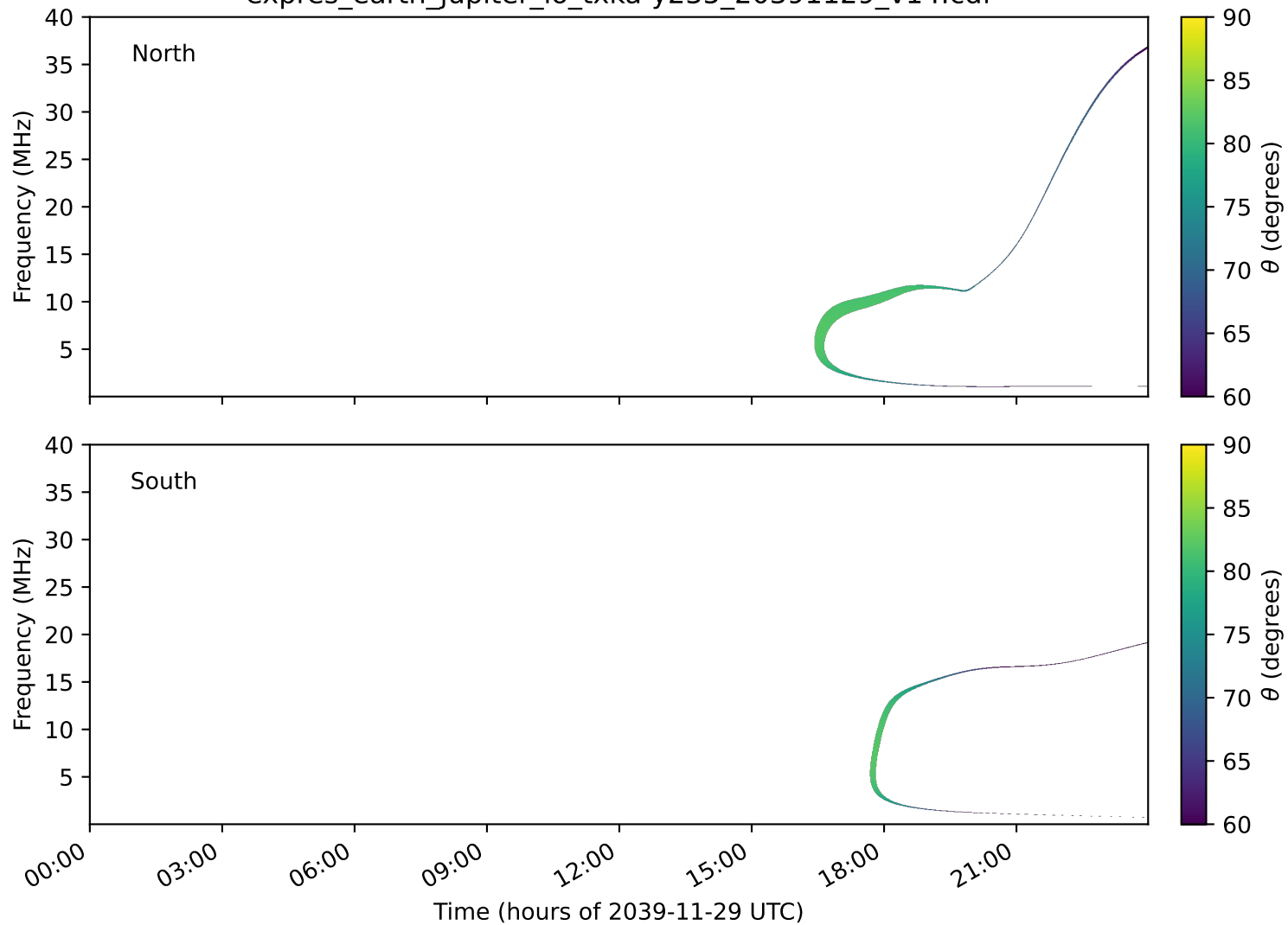
expres_earth_jupiter_io_txka-y235_20391129_v14.cdf
