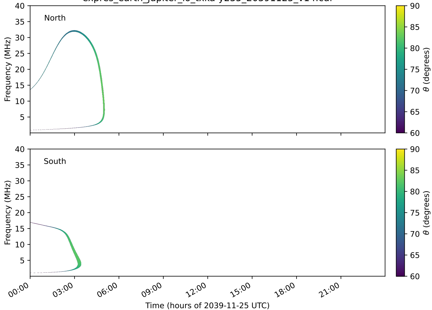
expres_earth_jupiter_io_txka-y235_20391125_v14.cdf
