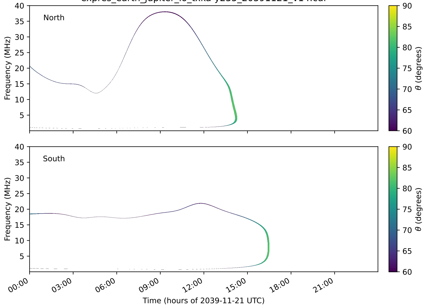
expres_earth_jupiter_io_txka-y235_20391121_v14.cdf
