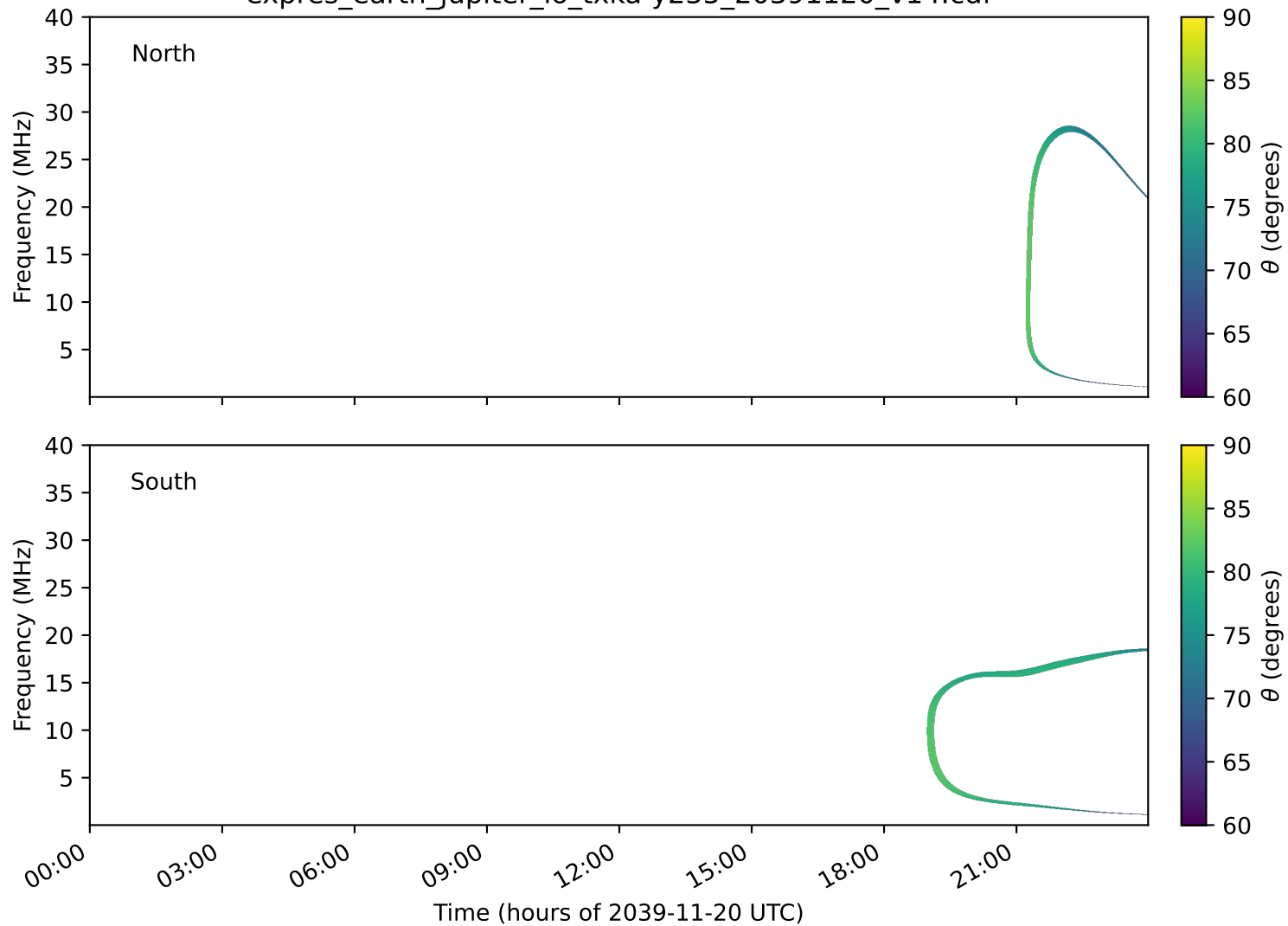
expres_earth_jupiter_io_txka-y235_20391120_v14.cdf
