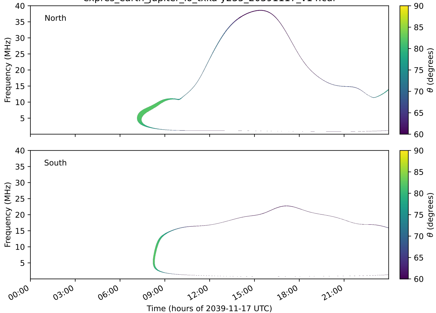
expres_earth_jupiter_io_txka-y235_20391117_v14.cdf
