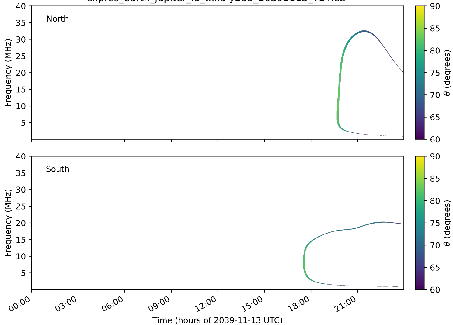
expres_earth_jupiter_io_txka-y235_20391113_v14.cdf
