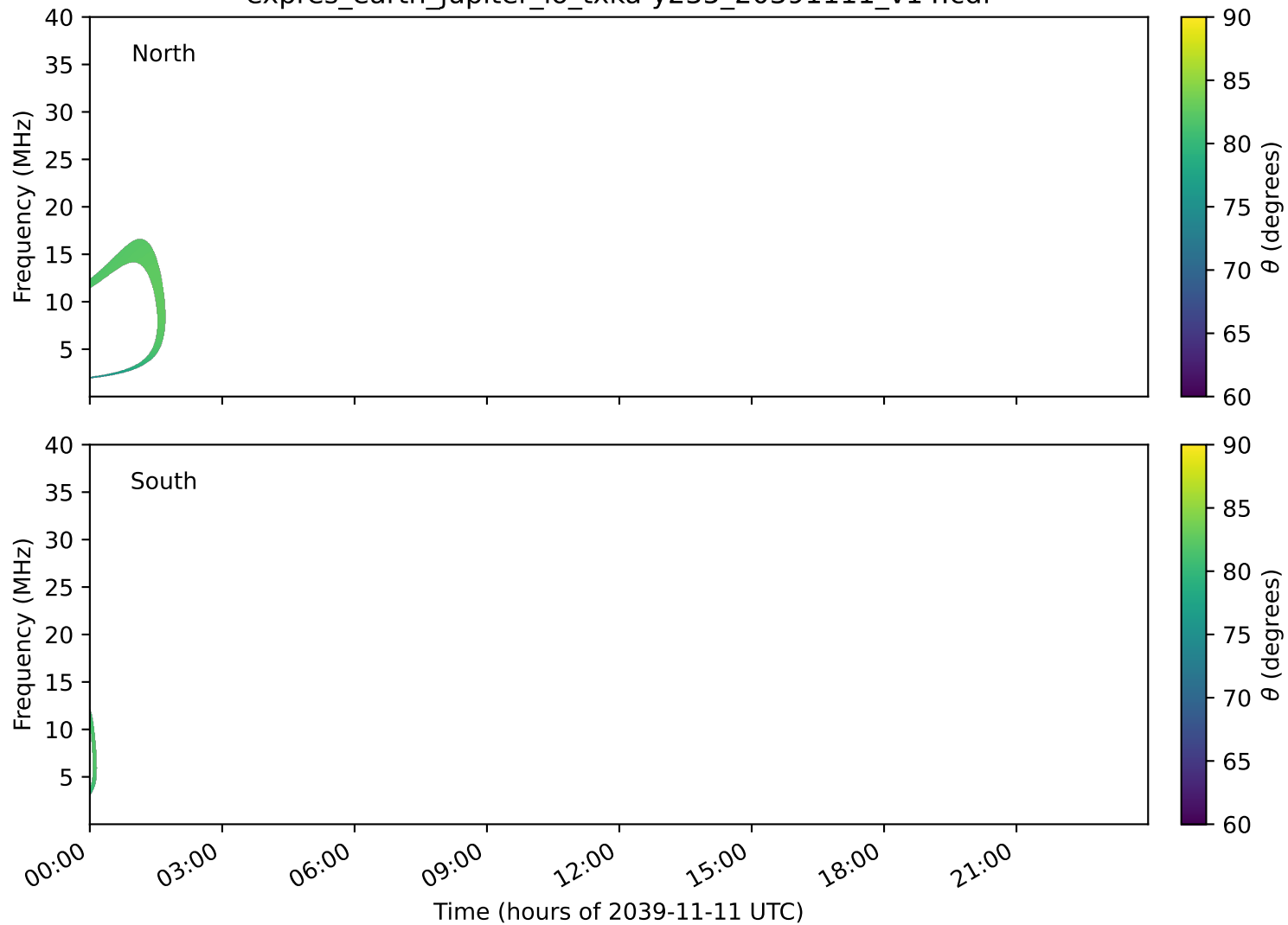
expres_earth_jupiter_io_txka-y235_20391111_v14.cdf
