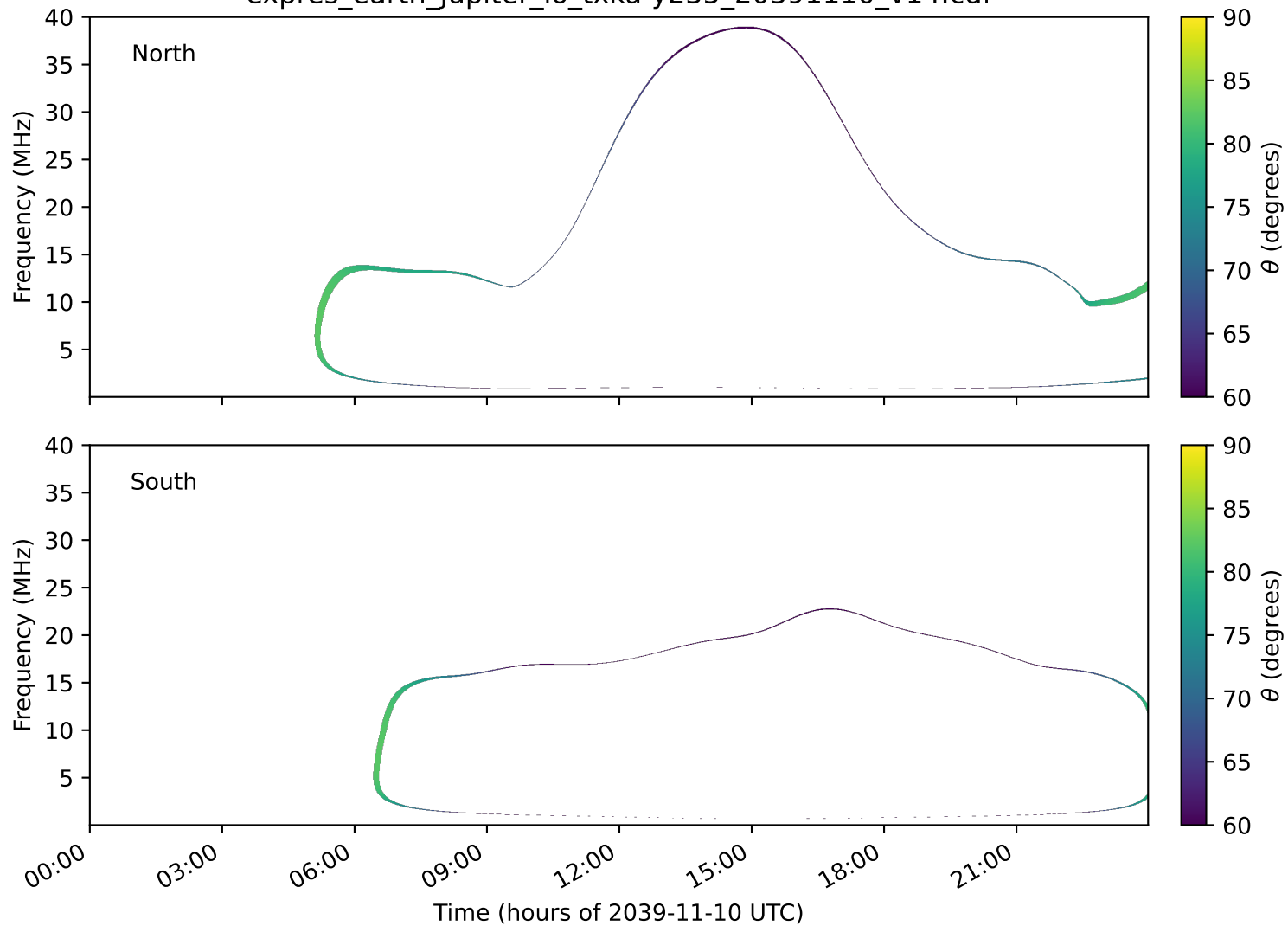
expres_earth_jupiter_io_txka-y235_20391110_v14.cdf
