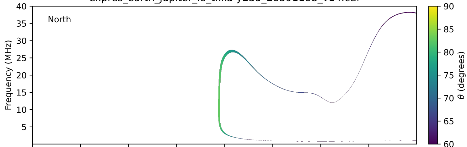
expres_earth_jupiter_io_txka-y235_20391108_v14.cdf
