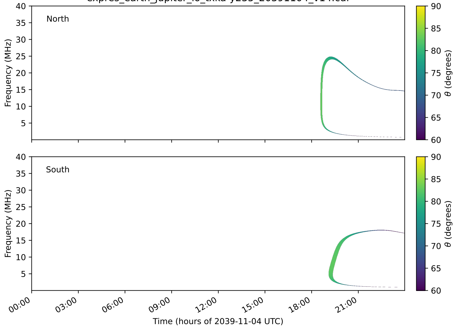
expres_earth_jupiter_io_txka-y235_20391104_v14.cdf
