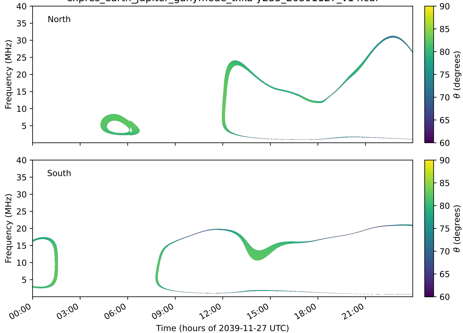
expres_earth_jupiter_ganymede_txka-y235_20391127_v14.cdf
