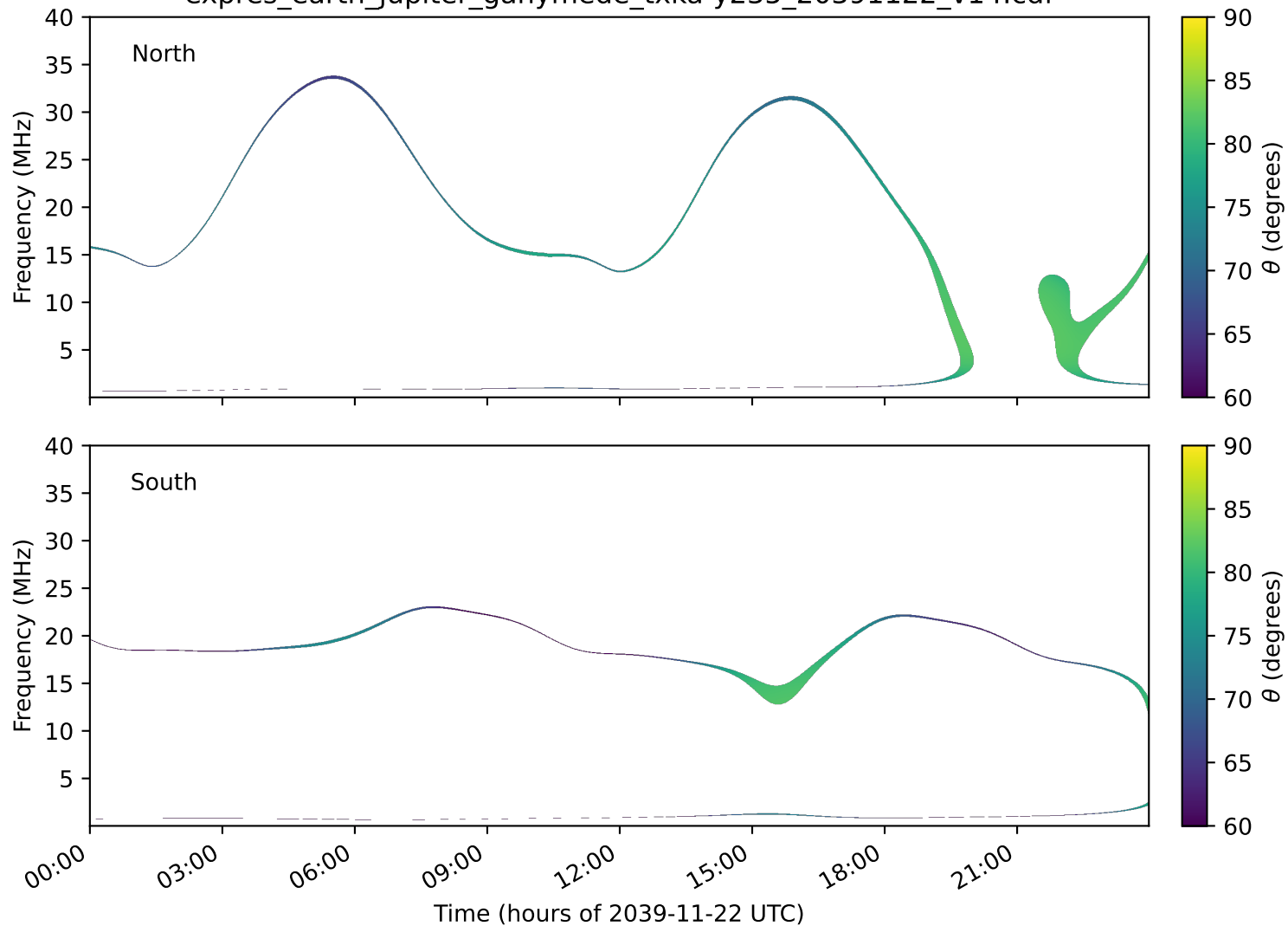
expres_earth_jupiter_ganymede_txka-y235_20391122_v14.cdf
