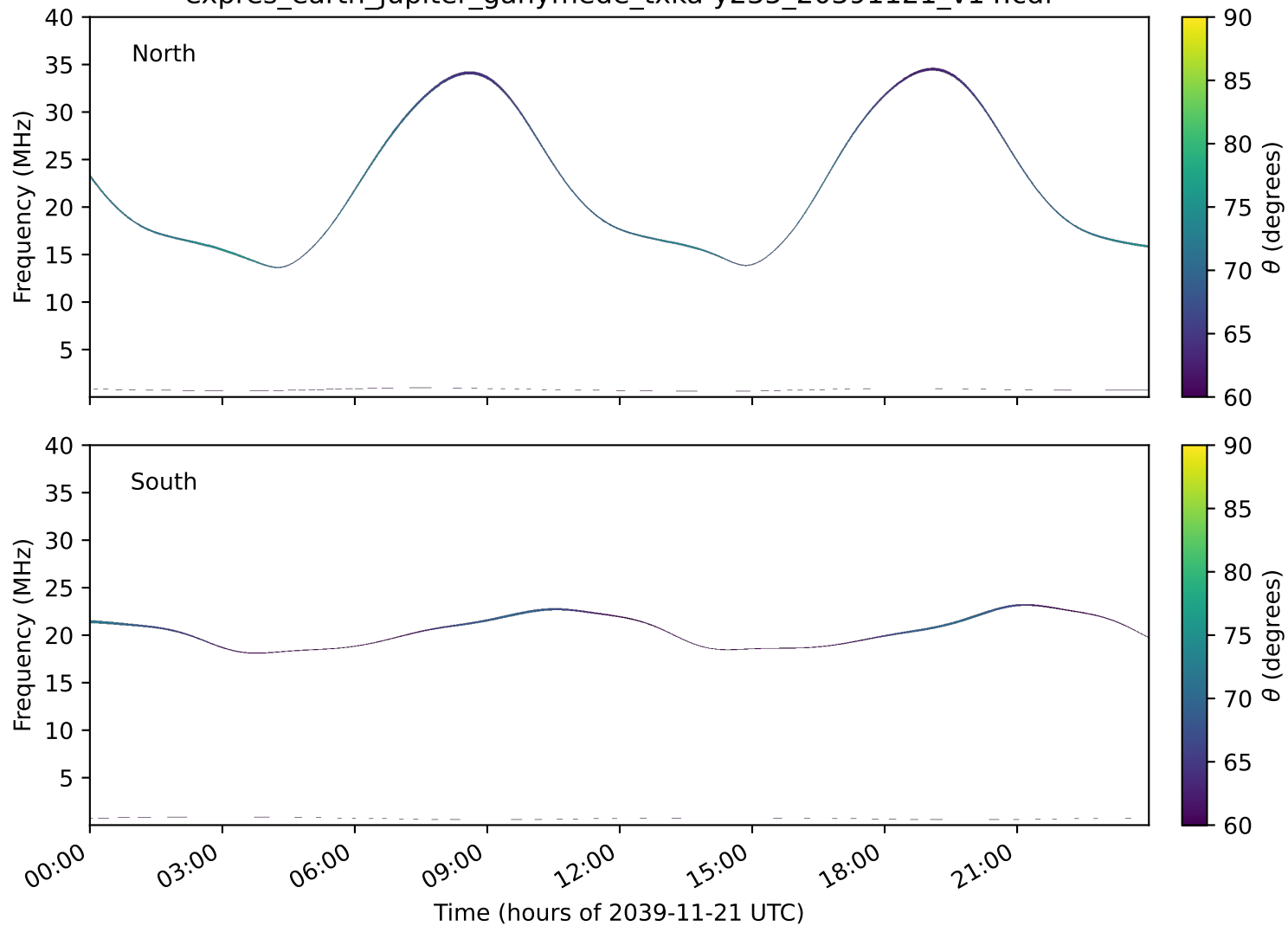
expres_earth_jupiter_ganymede_txka-y235_20391121_v14.cdf
