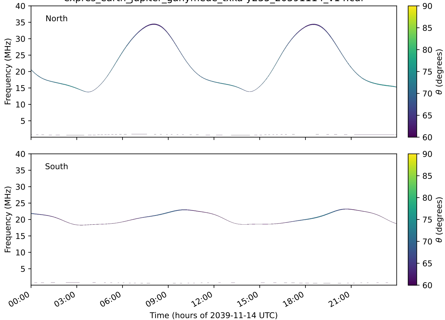
expres_earth_jupiter_ganymede_txka-y235_20391114_v14.cdf
