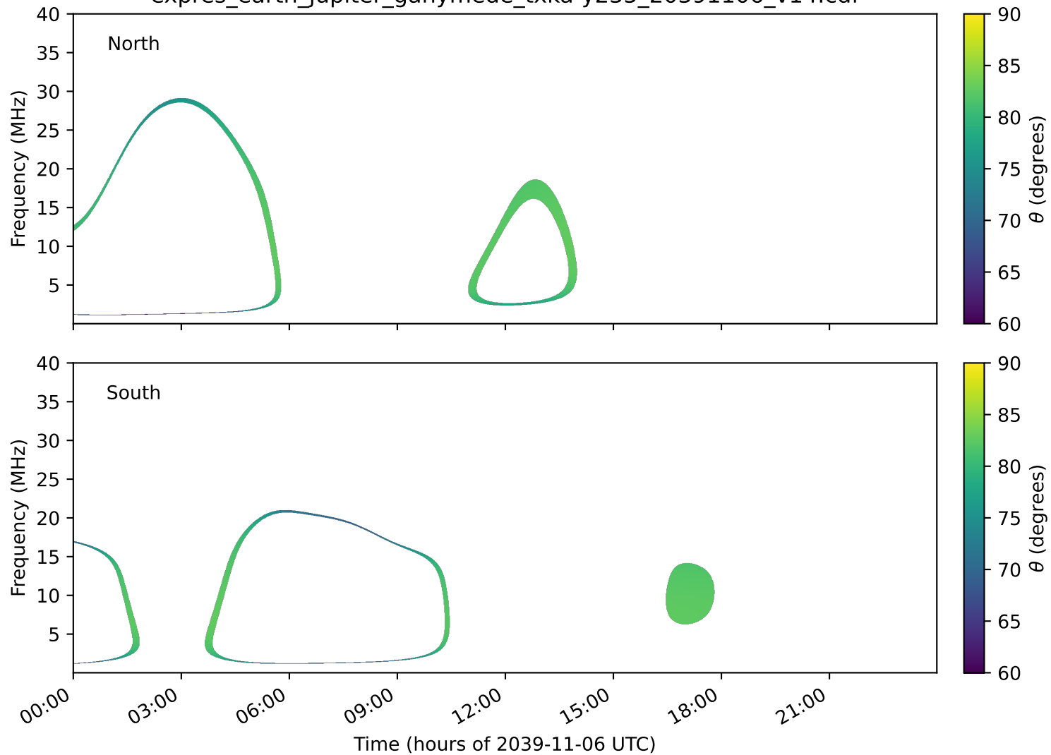
expres_earth_jupiter_ganymede_txka-y235_20391106_v14.cdf
