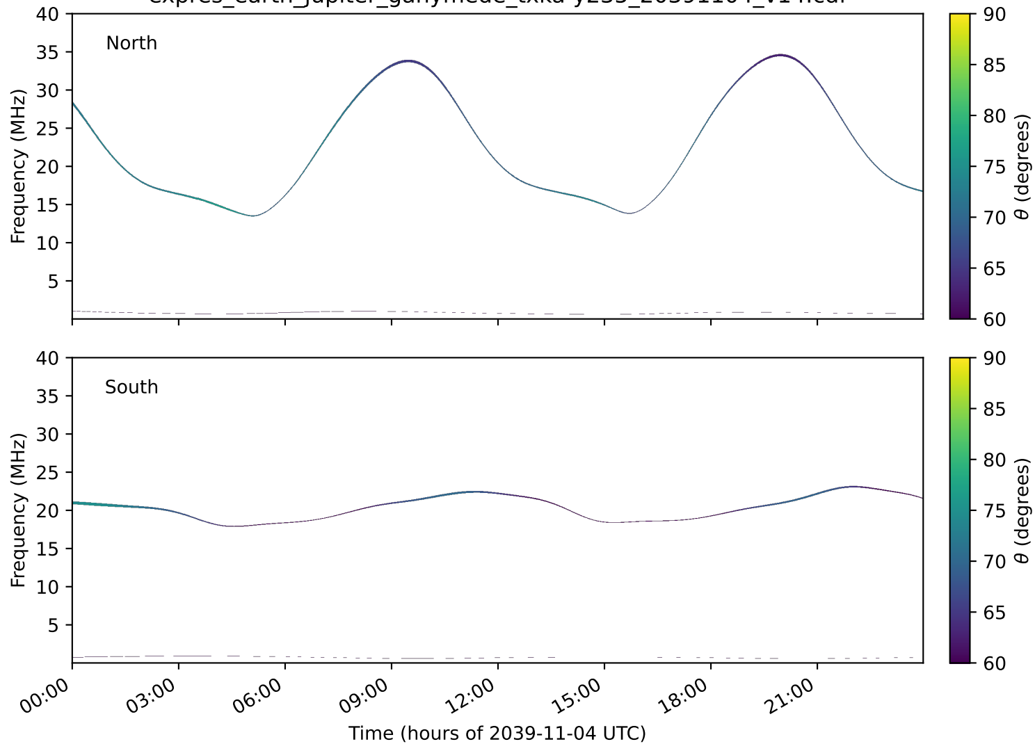
expres_earth_jupiter_ganymede_txka-y235_20391104_v14.cdf
