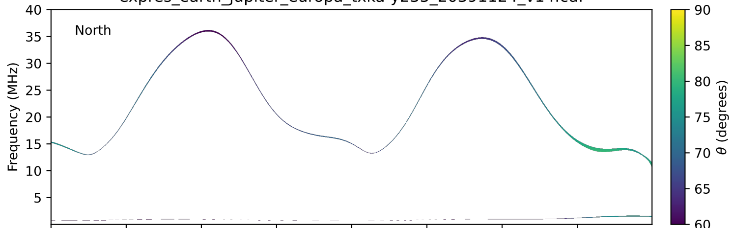
expres_earth_jupiter_europa_txka-y235_20391124_v14.cdf
