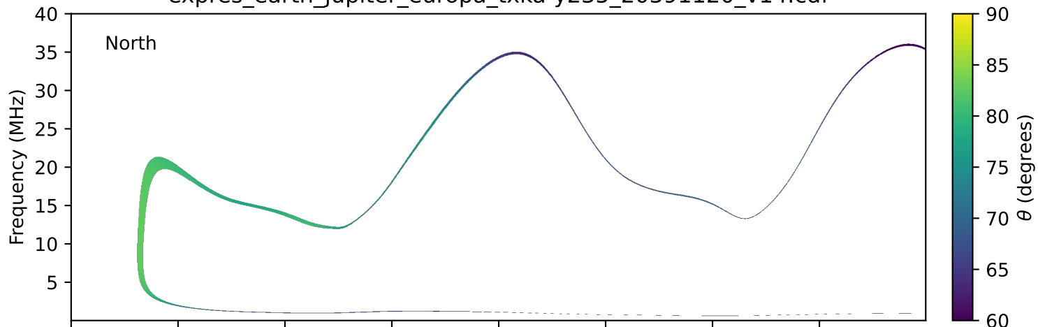
expres_earth_jupiter_europa_txka-y235_20391120_v14.cdf
