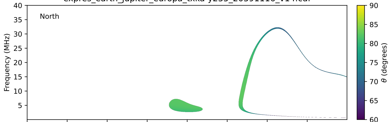
expres_earth_jupiter_europa_txka-y235_20391116_v14.cdf
