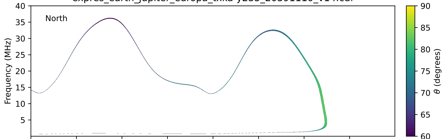
expres_earth_jupiter_europa_txka-y235_20391110_v14.cdf
