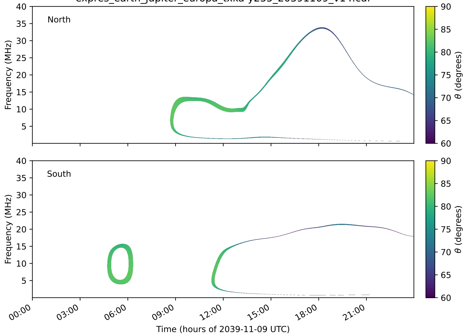
expres_earth_jupiter_europa_txka-y235_20391109_v14.cdf
