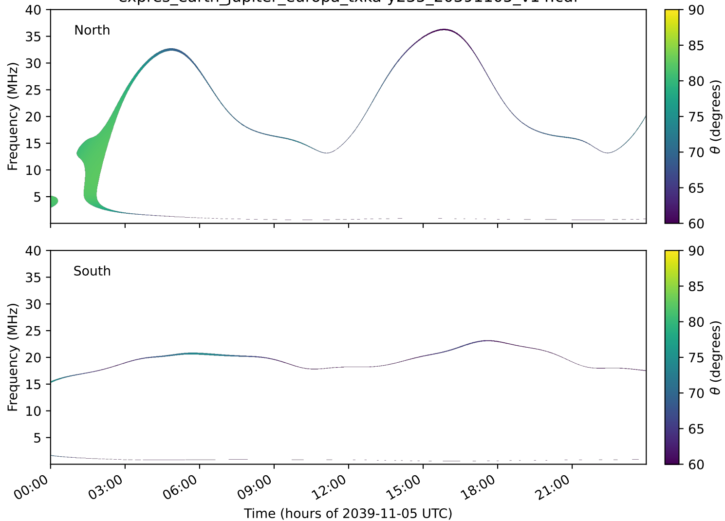
expres_earth_jupiter_europa_txka-y235_20391105_v14.cdf
