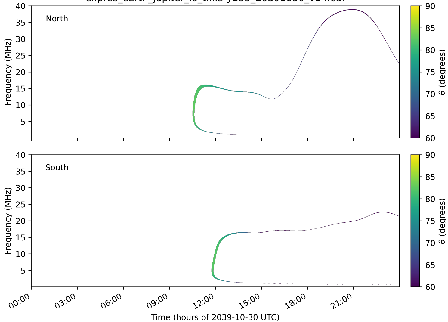
expres_earth_jupiter_io_txka-y235_20391030_v14.cdf
