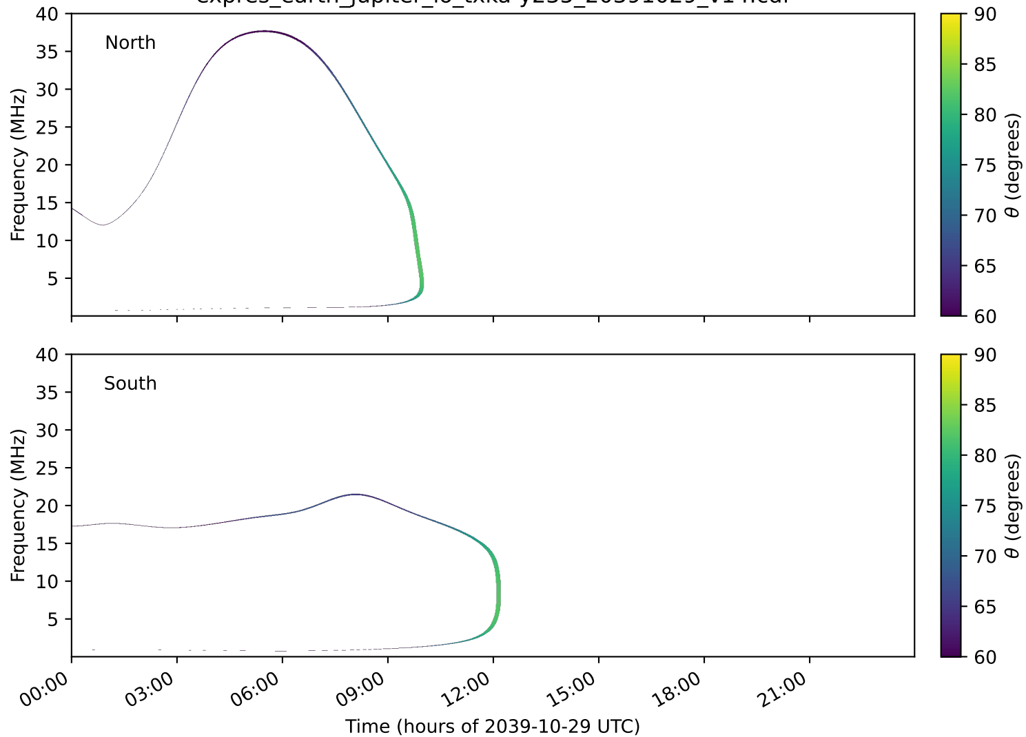
expres_earth_jupiter_io_txka-y235_20391029_v14.cdf
