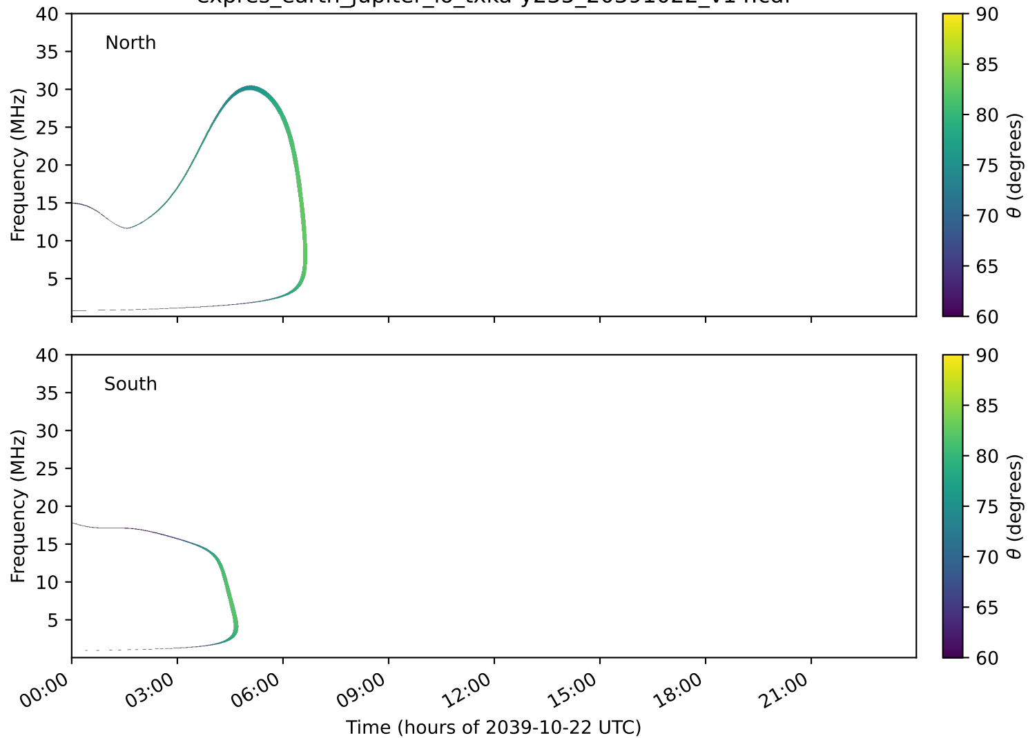
expres_earth_jupiter_io_txka-y235_20391022_v14.cdf
