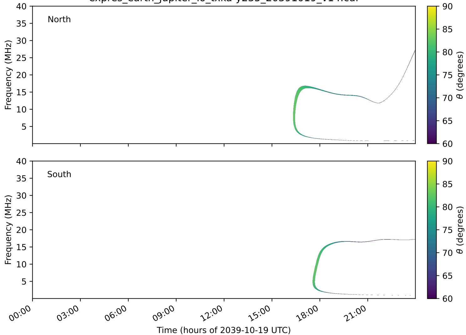
expres_earth_jupiter_io_txka-y235_20391019_v14.cdf
