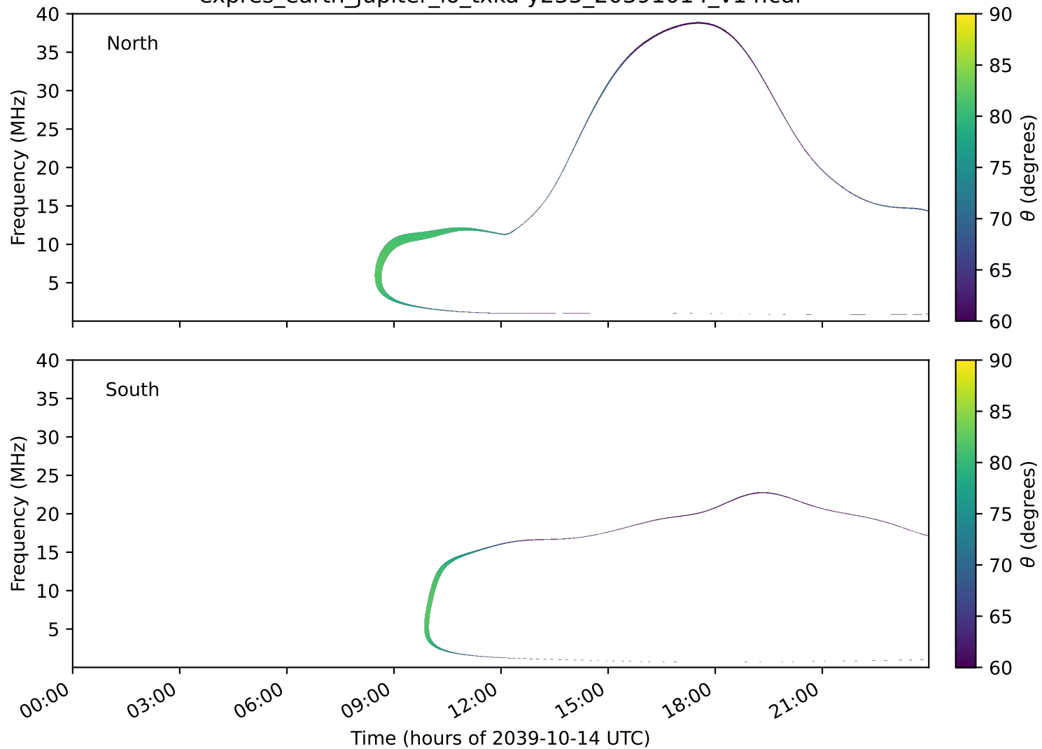
expres_earth_jupiter_io_txka-y235_20391014_v14.cdf
