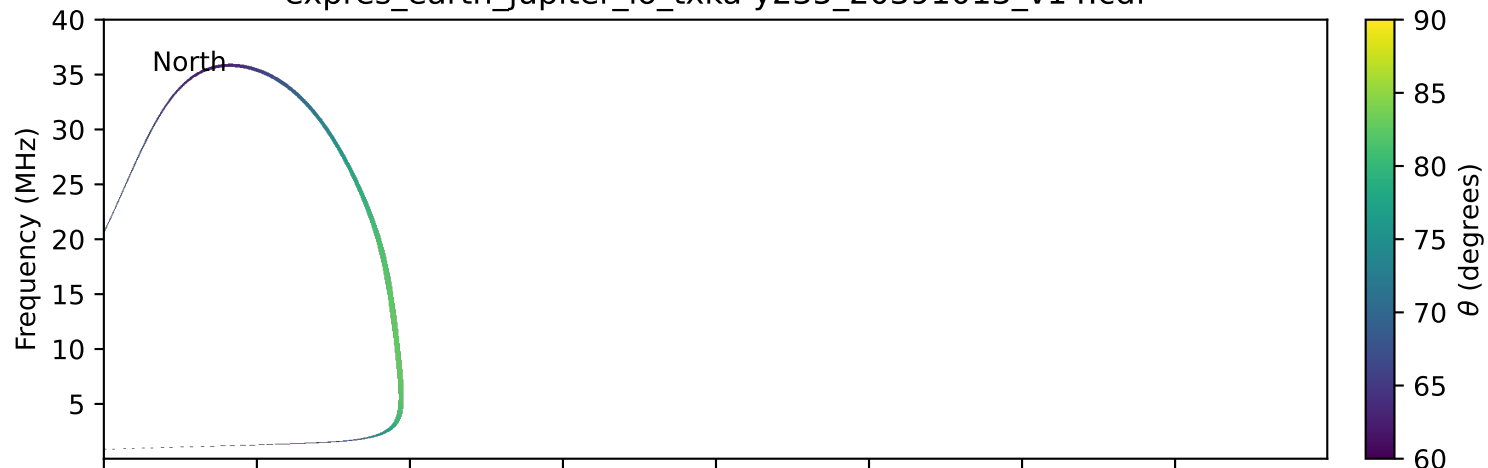
expres_earth_jupiter_io_txka-y235_20391013_v14.cdf
