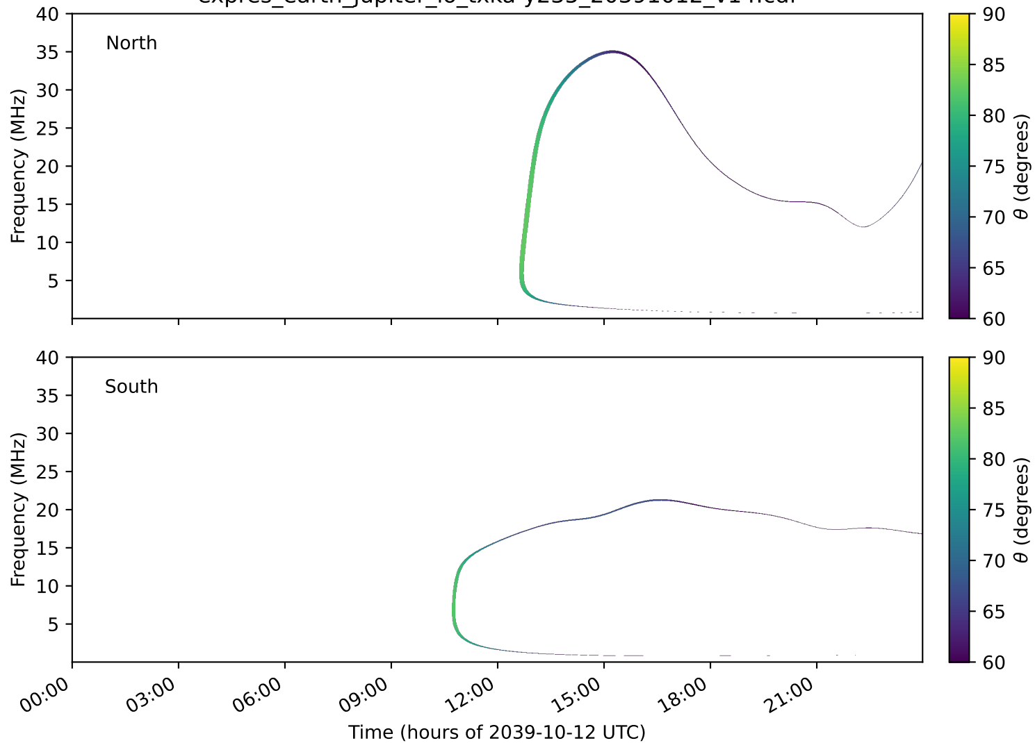
expres_earth_jupiter_io_txka-y235_20391012_v14.cdf
