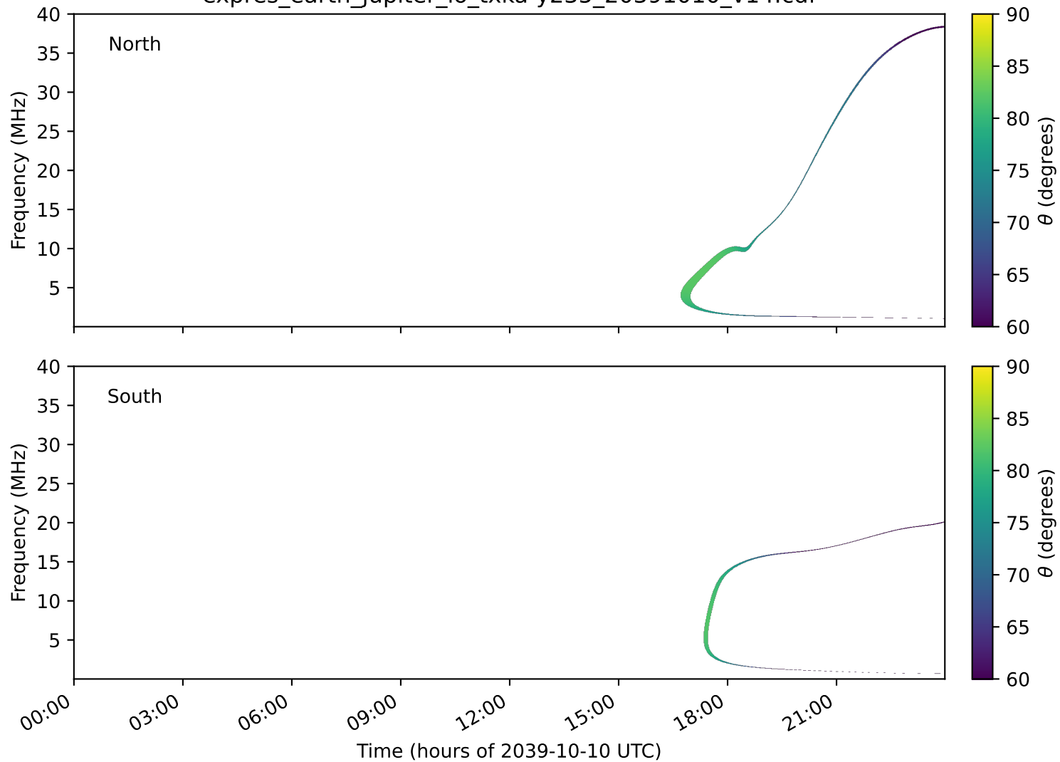
expres_earth_jupiter_io_txka-y235_20391010_v14.cdf
