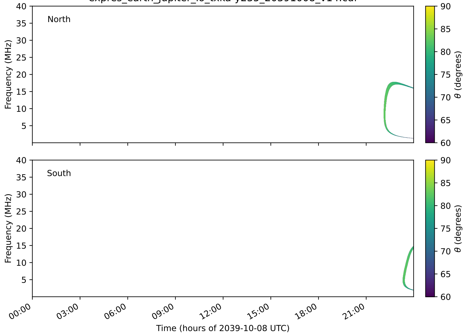
expres_earth_jupiter_io_txka-y235_20391008_v14.cdf
