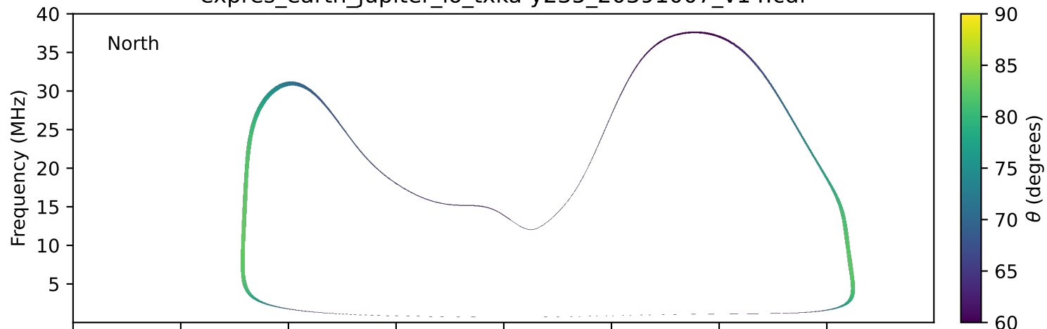
expres_earth_jupiter_io_txka-y235_20391007_v14.cdf
