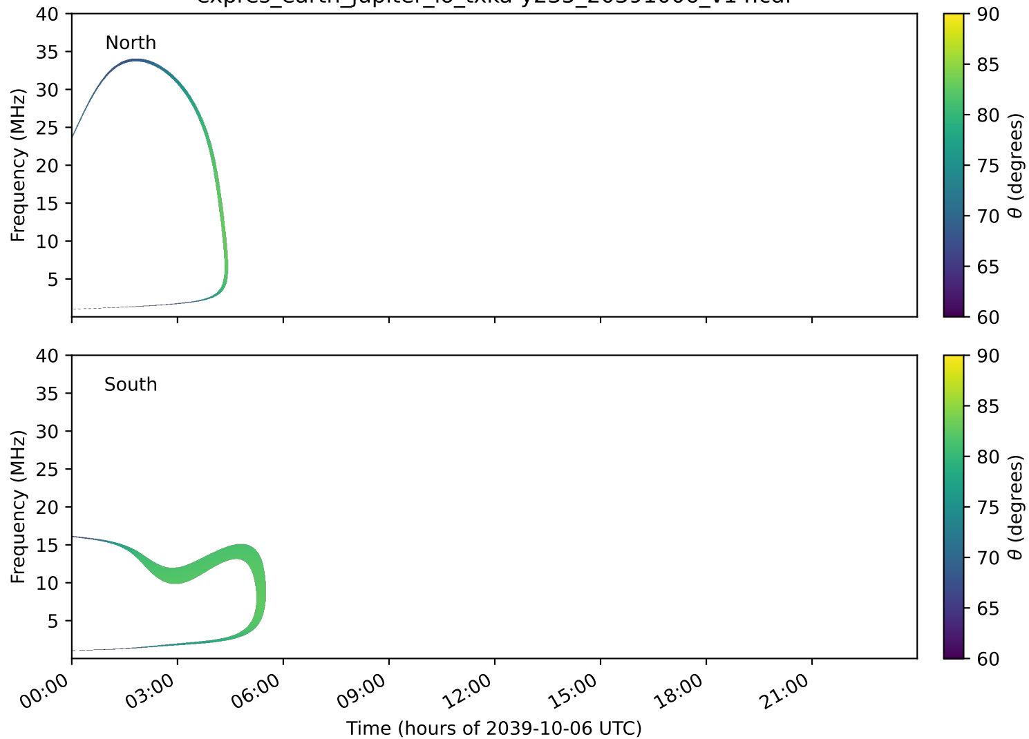
expres_earth_jupiter_io_txka-y235_20391006_v14.cdf
