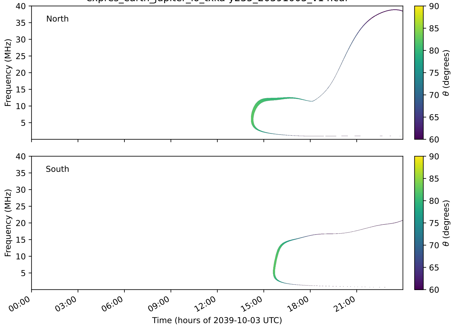
expres_earth_jupiter_io_txka-y235_20391003_v14.cdf
