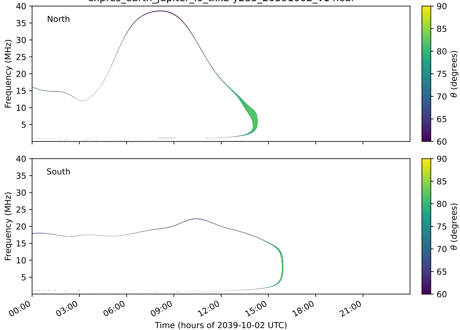
expres_earth_jupiter_io_txka-y235_20391002_v14.cdf
