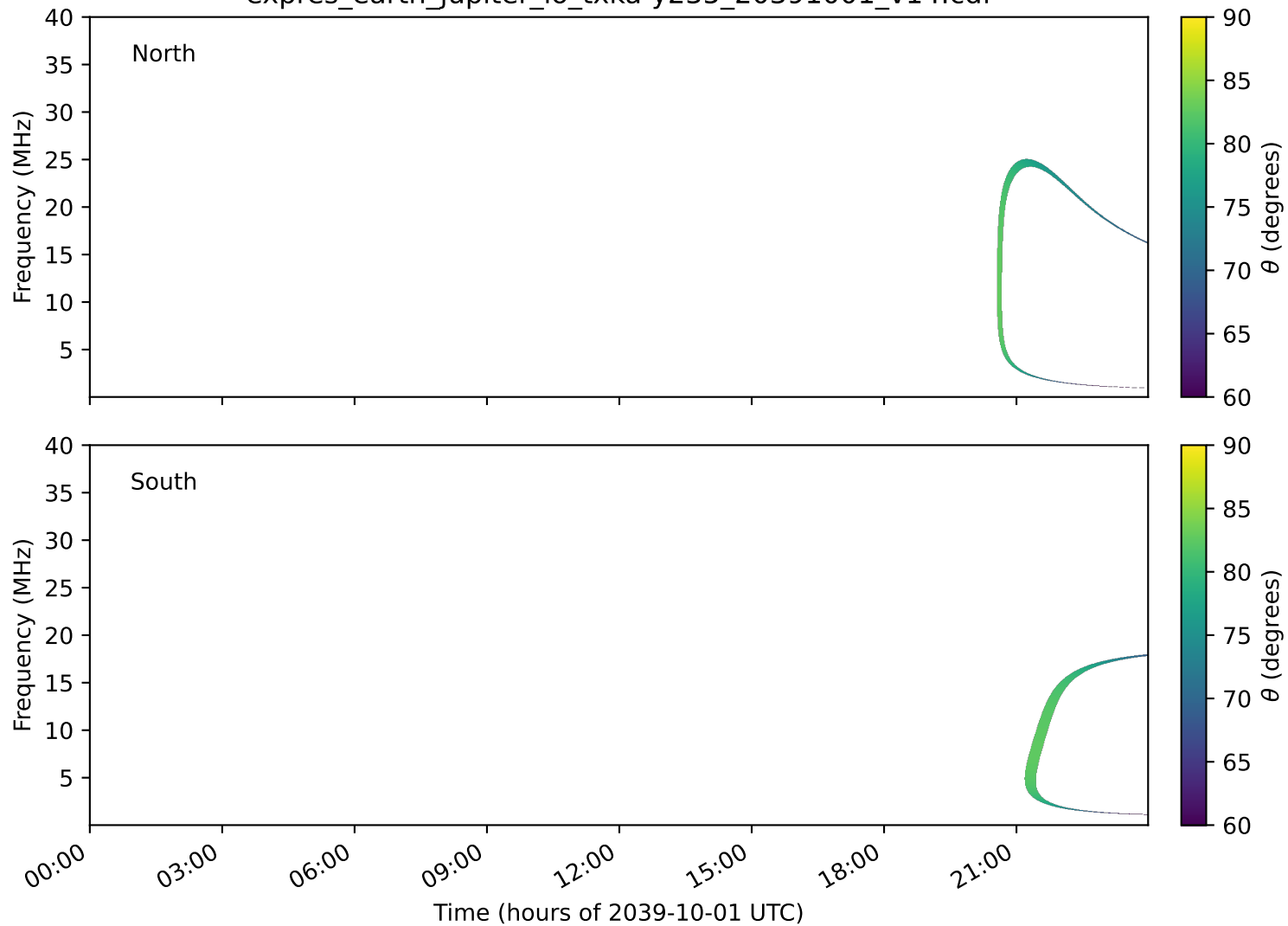
expres_earth_jupiter_io_txka-y235_20391001_v14.cdf
