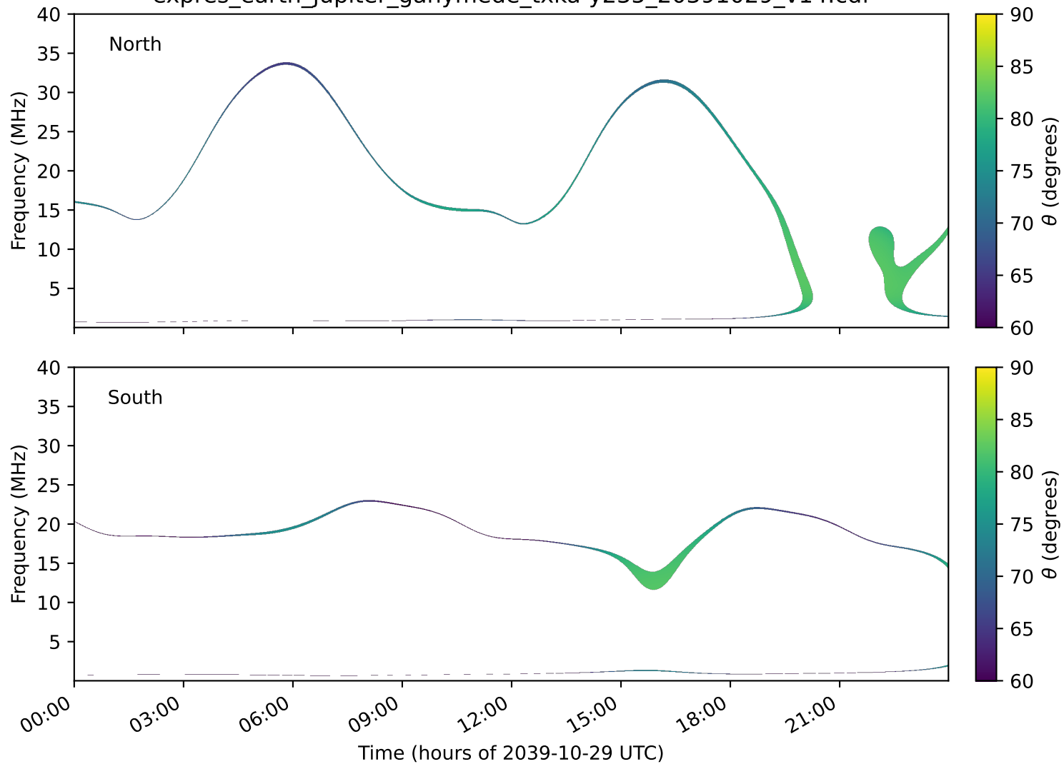
expres_earth_jupiter_ganymede_txka-y235_20391029_v14.cdf
